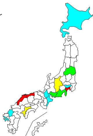
67 例 Coxsackievirus A16
